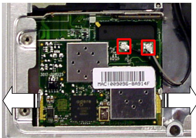
Fig. 16 Wireless Card Module
